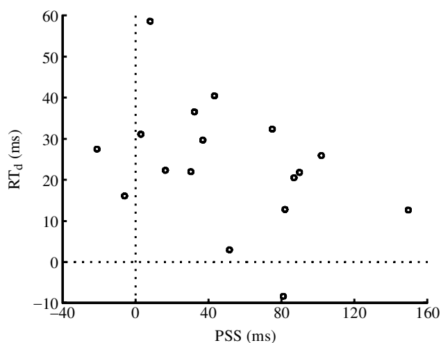
Figure 2. Plot of PSS versus RT_d for the 17 observers in experiment 1.
